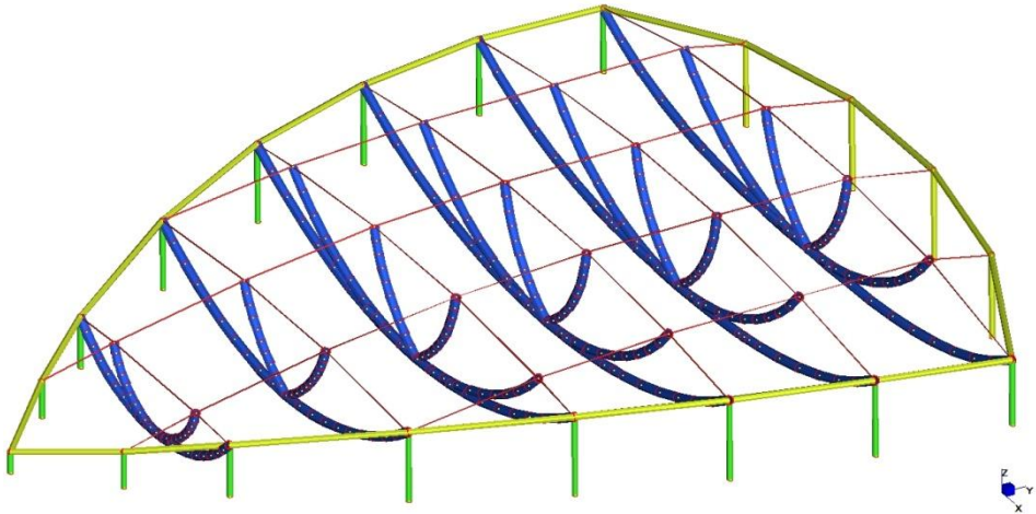
Figure 7: Finite Element Model of the steel structure.
